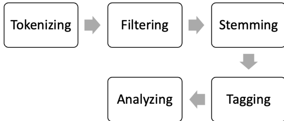
Figure 1. Preprocessing Text
