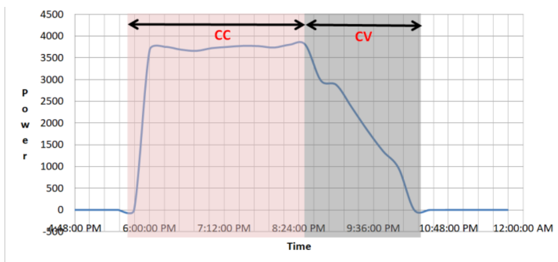
Figure 3. Power profile of PEV charging
