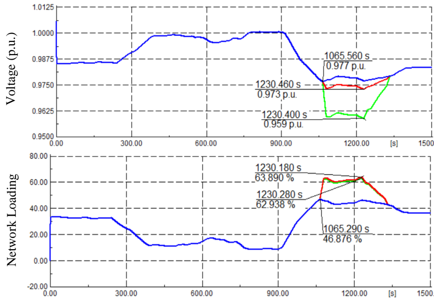
Figure 7. Voltage and feeder loading impact of PEV charging location
