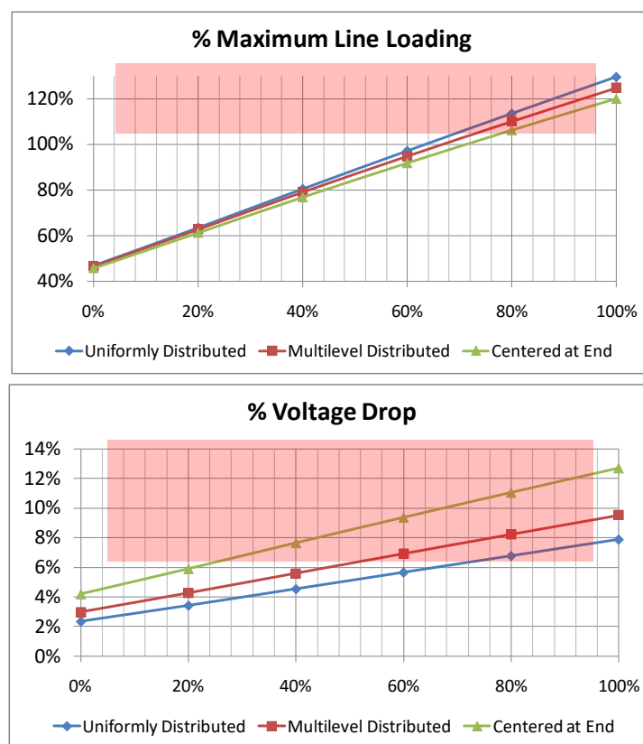
Figure 8. Impact of PEV penetration on maximum line loading and voltage drop
