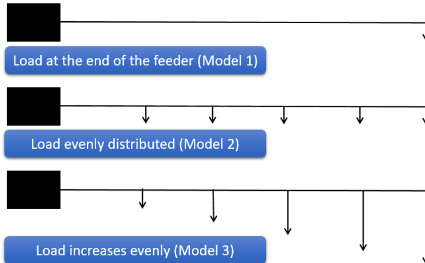
Figure 2. Model of distributed load in the distribution network
