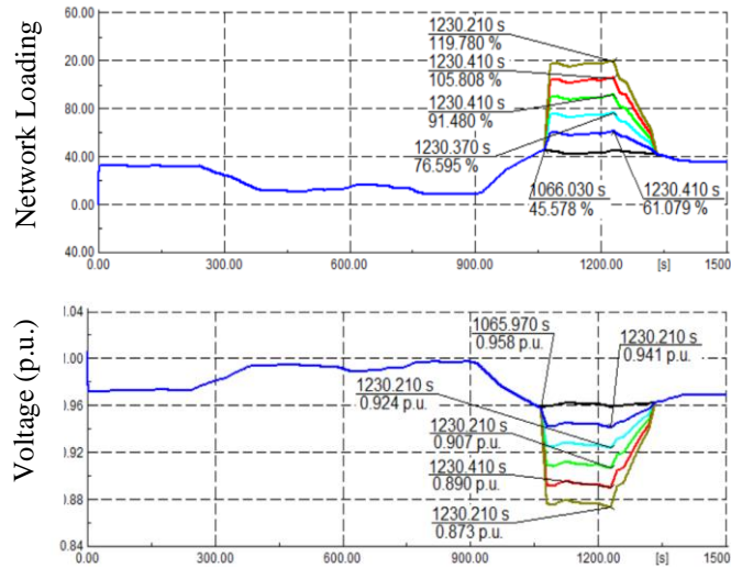
Figure 4. Feeder loading and voltage drop of distribution network model 1
