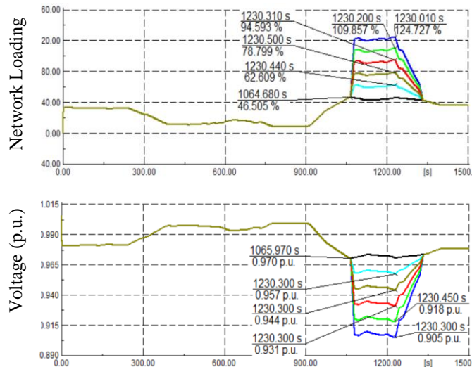
Figure 6. Feeder loading and voltage drop of distribution network model 3
