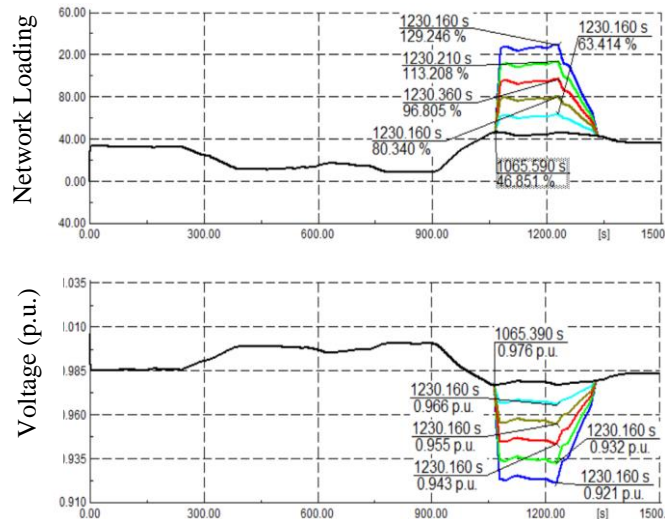
Figure 5. Feeder loading and voltage drop of distribution network model 2
