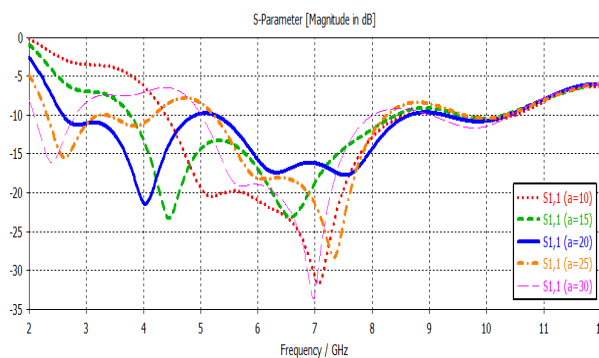
Fig. 5. S_{11} results on variations in antenna length
