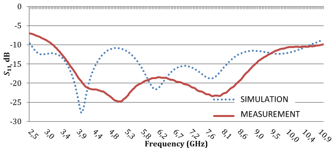
Fig. 9. Comparison between S11 simulation and measurement
