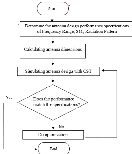
Fig. 2. Flowchart Monopole Antenna Design
