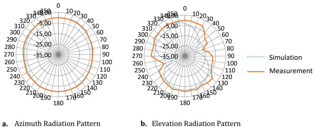
Fig. 10. Comparison radiation pattern
