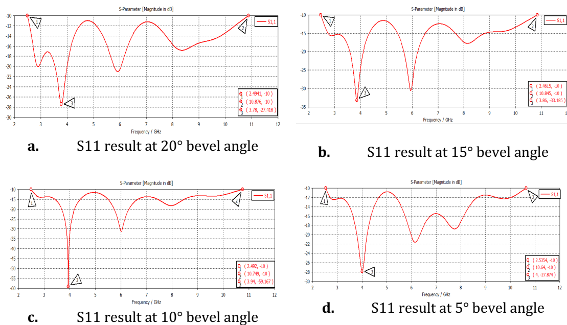
Fig. 7. S11 result with variation bevel angle
