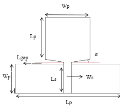
a. Monopole antenna final design
