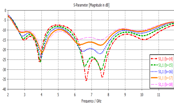
Fig. 6. S_{11} results on variations in antenna width
