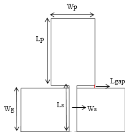
Fig. 3. Initial Monopole Antenna Design
