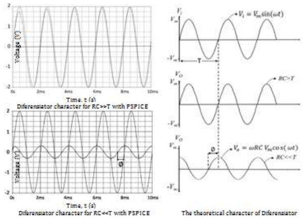
Figure 6. The differential character with sine wave input
