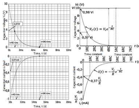
Figure 2. Comparison of voltage curves and current discharging capacitors SPICE virtual laboratory experiment results and theoretical.
