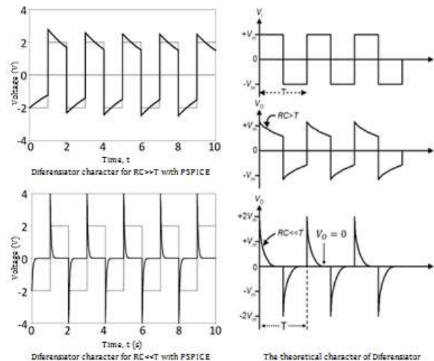
Figure 5. Differentiator character with square wave input
