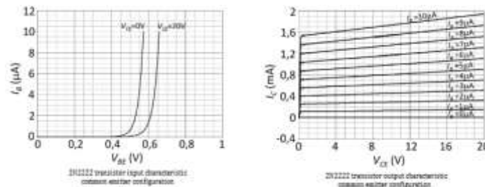
Figure 13. Characteristics of 2N2222 transistor with PSPICE
