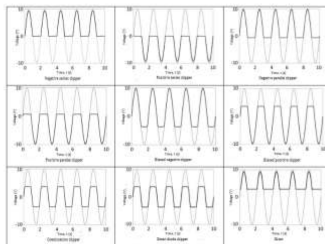
Figure 9. Character of a wave-forming circuit
