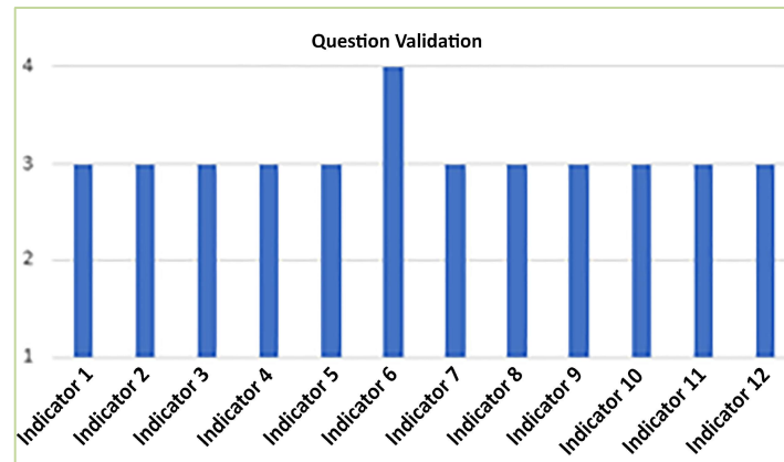
Figure 3. Question Validation
