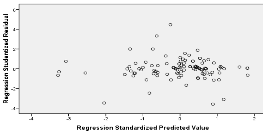
Figure 2. Heteroskedasticity Test Results
