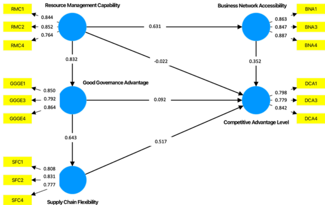
Figure 2. Measurement Outer Loading Model
