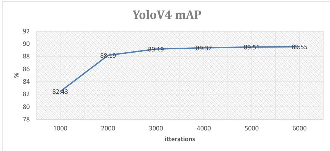
Figure 4. Yolo V4 Mean Average Precision
