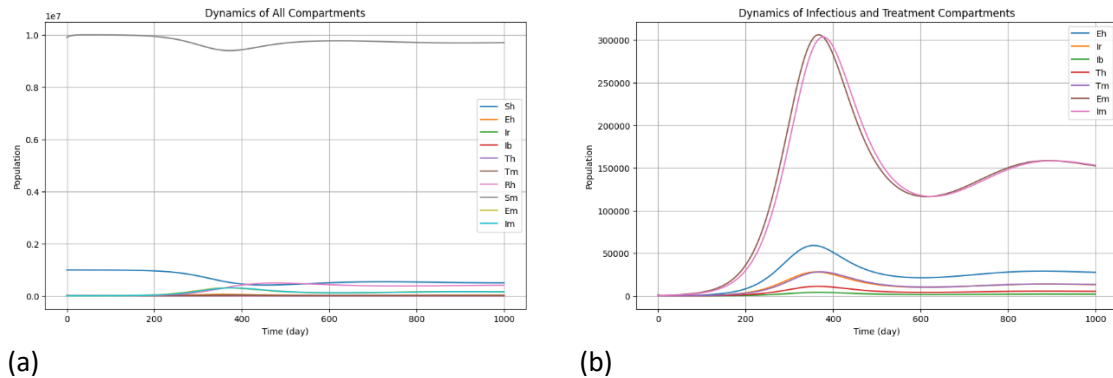
(a) (b) Figure 3. Numerical simulation for Case 2 ( \tau_h = 0.1 , \phi = 0.2 ). (a) Dynamics of All Compartments, (b) Dynamics of Infectious and Treatment Compartments.
