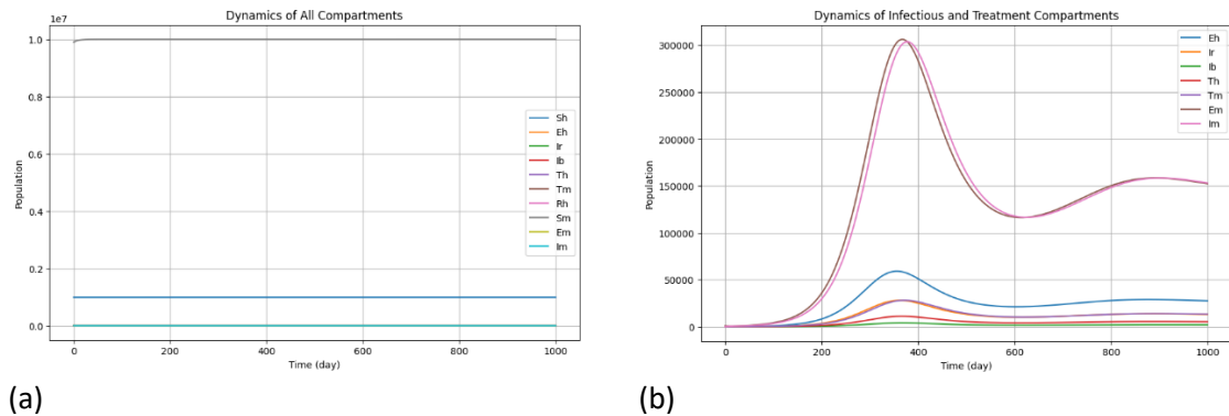
Figure 4. Numerical simulation for Case 3 ( \tau_h = 0.4 , \phi = 0.01 ). (a) Dynamics of All Compartments, (b) Dynamics of Infectious and Treatment Compartments.
