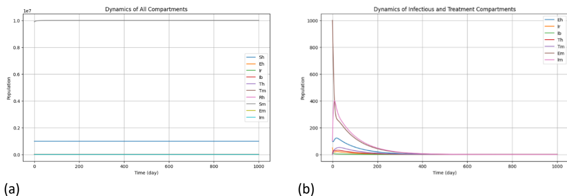
Figure 5. Numerical simulation for Case 4 ( \tau_h = 0.4 , \phi = 0.2 ). (a) Dynamics of All Compartments, (b) Dynamics of Infectious and Treatment Compartments.
