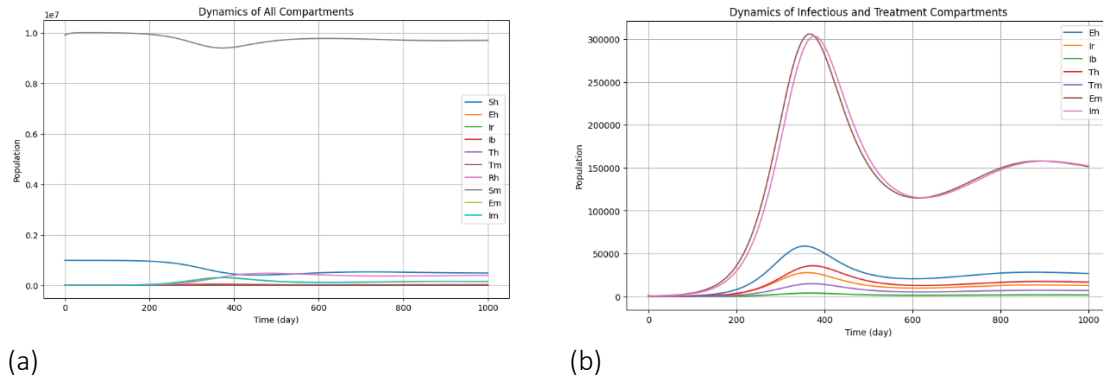
(a) (b) Figure 2. Numerical simulation for Case 1 ( \tau_h = 0.1 , \phi = 0.01 ). (a) Dynamics of All Compartments, (b) Dynamics of Infectious and Treatment Compartments.
